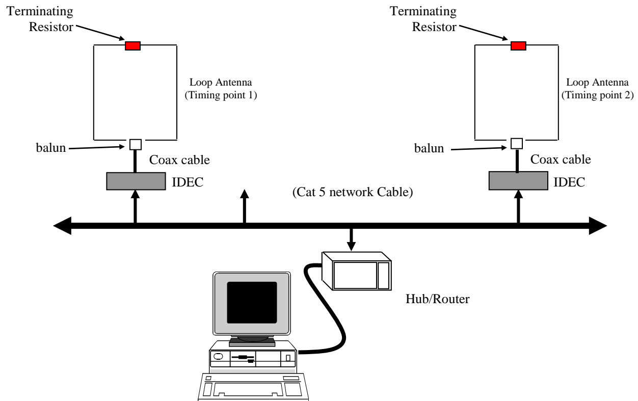
Fig 1.2 Multiple Timing Point Configuration
