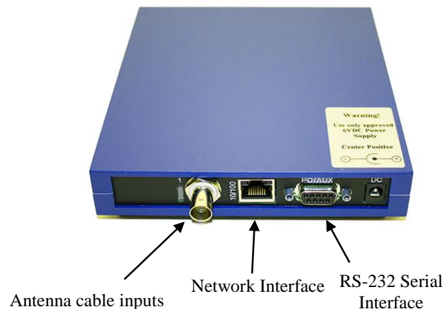
Fig. 2.2.1 IDEC Rear Panel (1 Port System)
